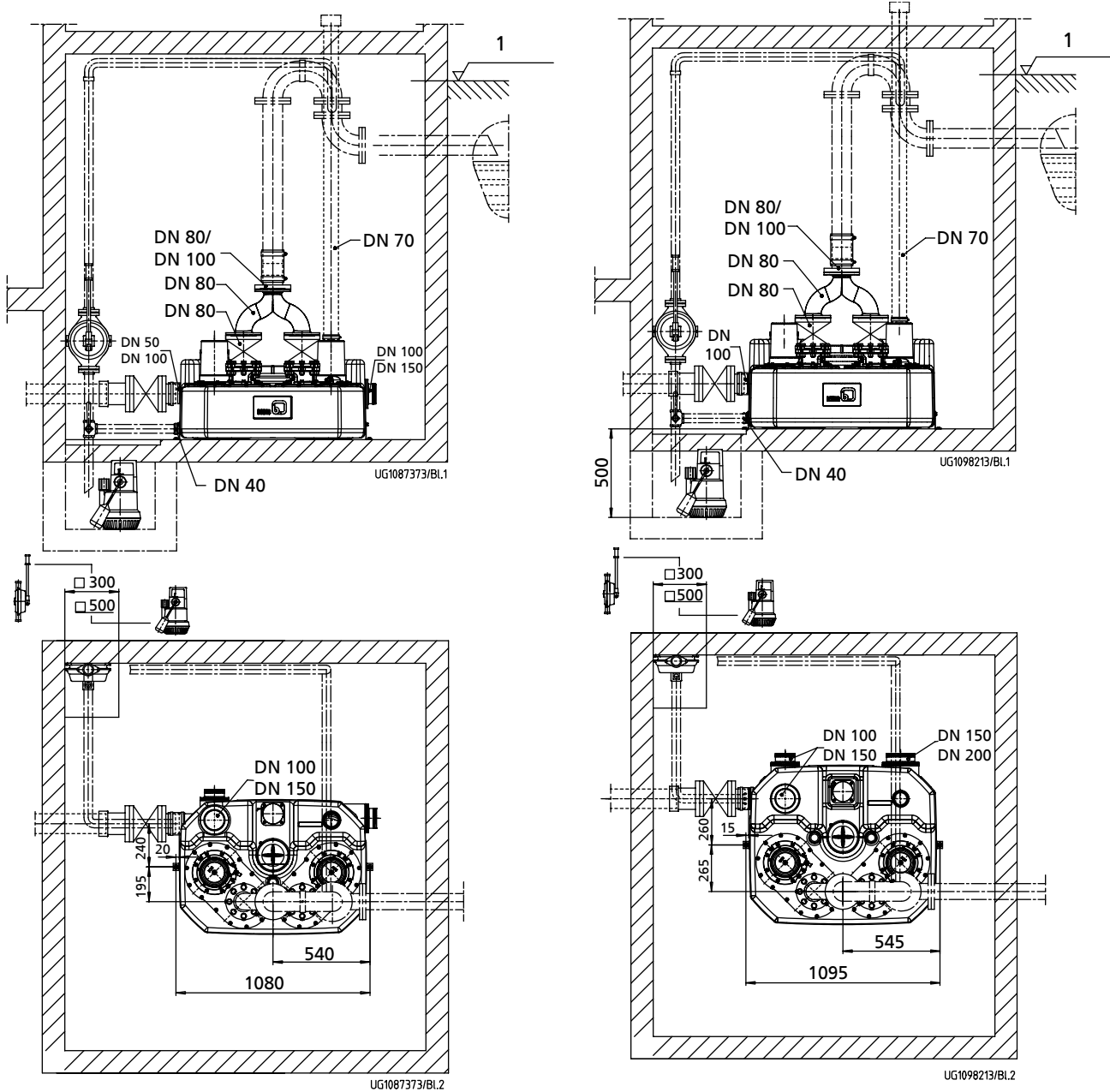
Compacta UZ150
