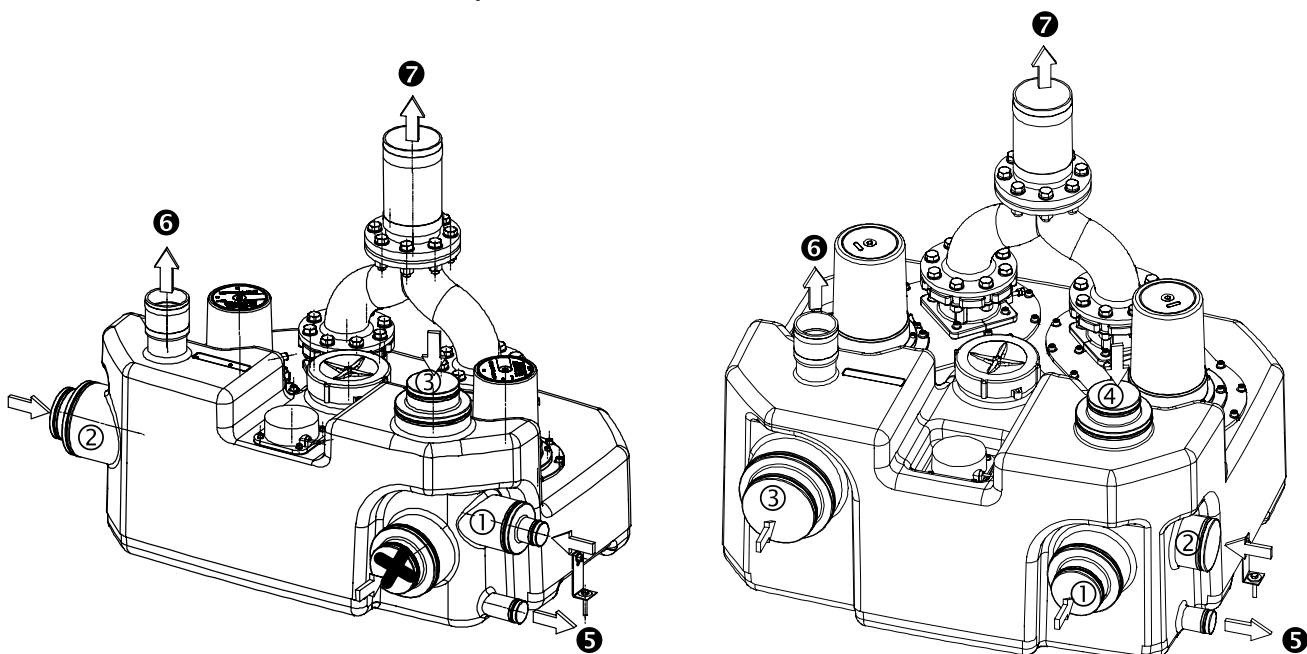
Compacta UZ150
