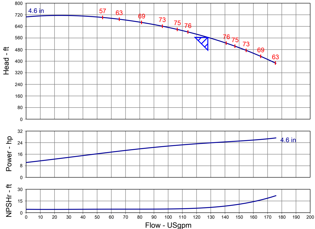
Performance based on test acceptance - ISO 9906:2012 3B. Performances are subject to periodic changes due to continuous improvements.
