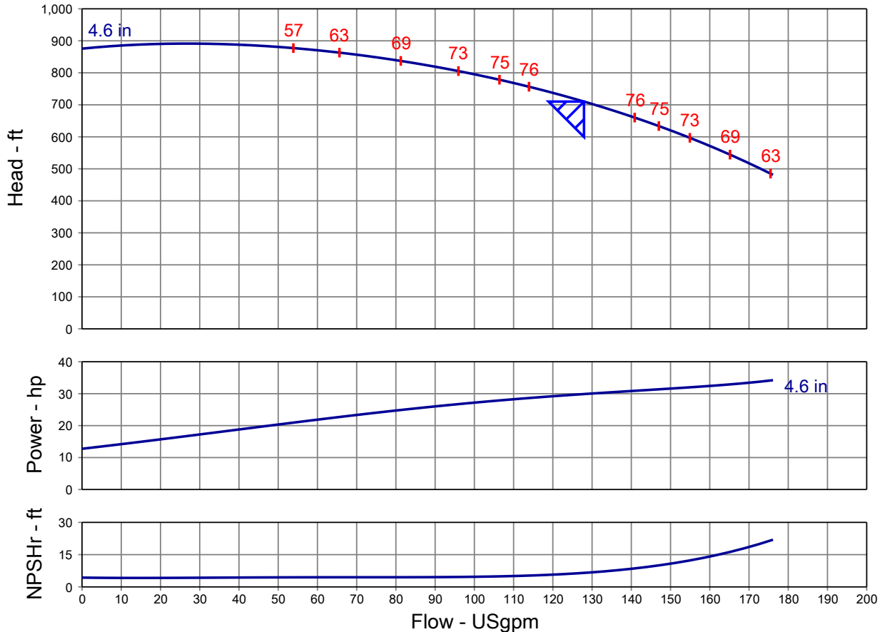
Performance based on test acceptance - ISO 9906:2012 3B. Performances are subject to periodic changes due to continuous improvements.
